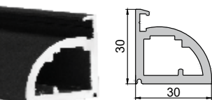
Frame Profile Profile Length: 3000mm
