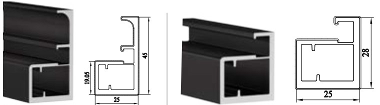
Handle Profile Profile Length: 3000mm Frame Profile Profile Length: 3000mm
