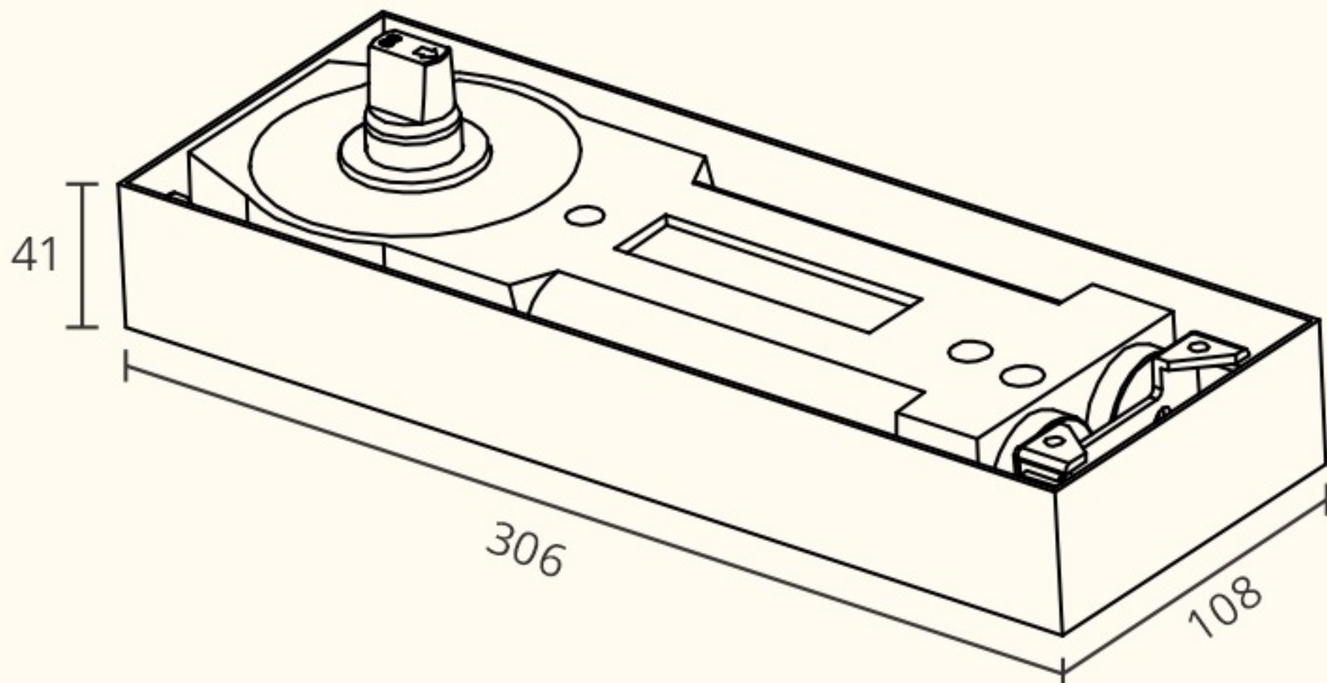
CUTOUT For 120 & 150 Kg Floor Spring
