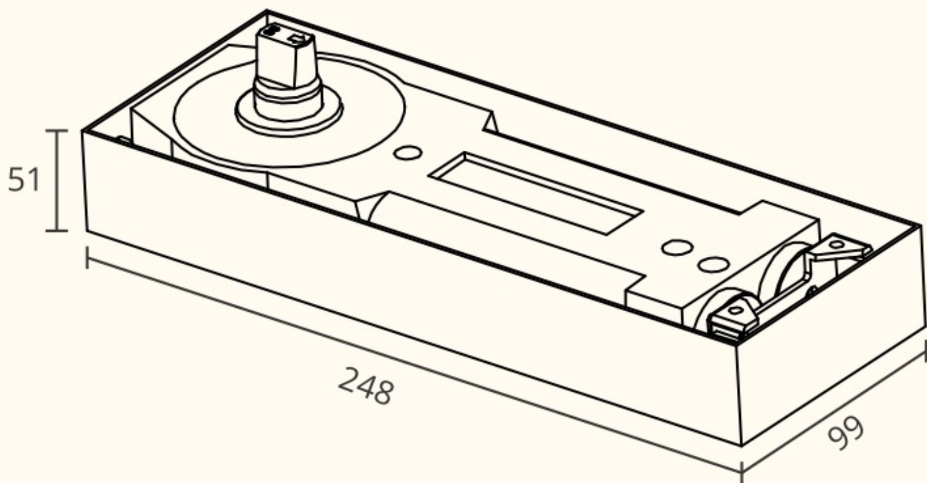
CUTOUT For 90 Kg Floor Spring
