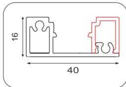
CASP-SHP-4016 (Clip M/F Set)
