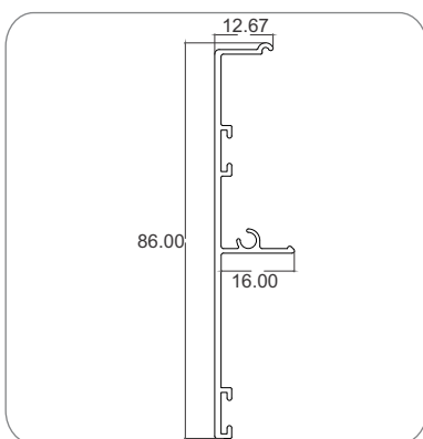
Track Cover CASP-TC-T1
