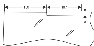
CDC-68 with Saddle Plate (187) with Door Width upto 1100mm
