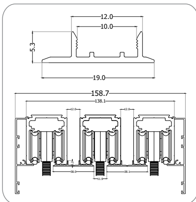
Top Track Concealer with Clip on : CASP-1411 (Optional)
