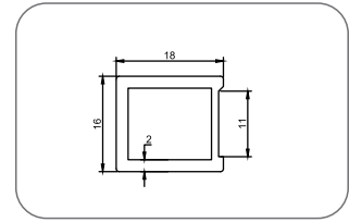
CASP-PB-1616 (Georgian Bar Heavy)
