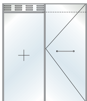
Ventilation Grill in Fix
