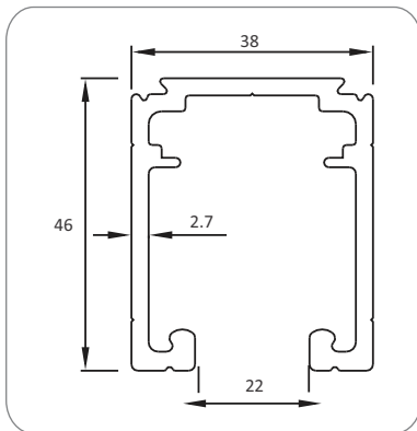
Top Track CASP-T1
