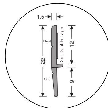
Water and Dustproof epdm Strip
