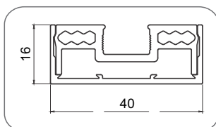
CASP-4006/07-4016 (Clip M/F Set)
