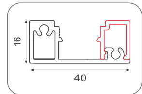
CASP-SHP-4016 (Clip M/F Set)
