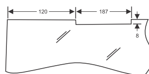
CDC-68 with Saddle Plate (187) with Door Width upto 950mm
